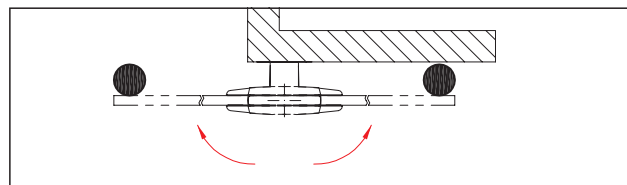
Fig. 1 Double-action door with on-site doorstops in any opening direction
