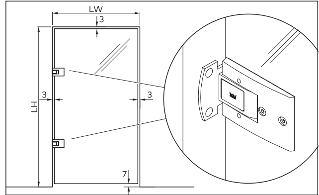
Fig. 5 Gaps for wall mounting with surface-mounted mounting plate
