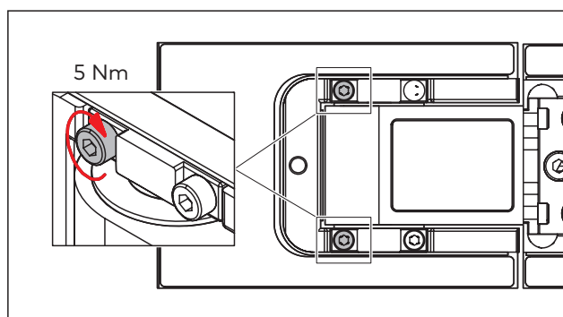
Fig. 29 Tighten the marked screws with torque.
