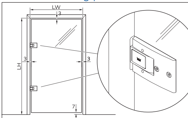
Fig. 8 Gaps for the frame with embedded mounting plate
