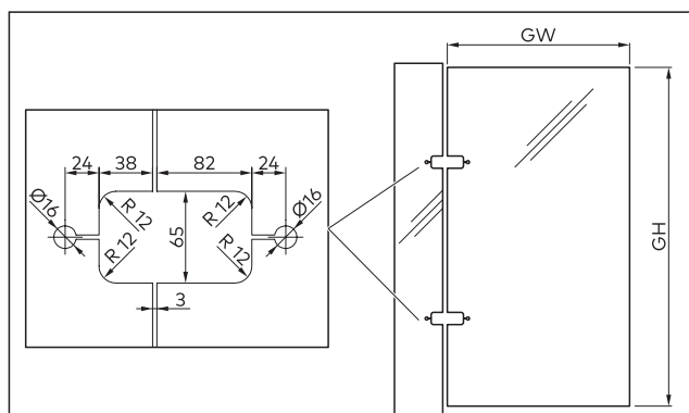
Fig. 13 Glass preparations for the glass to glass mounting
